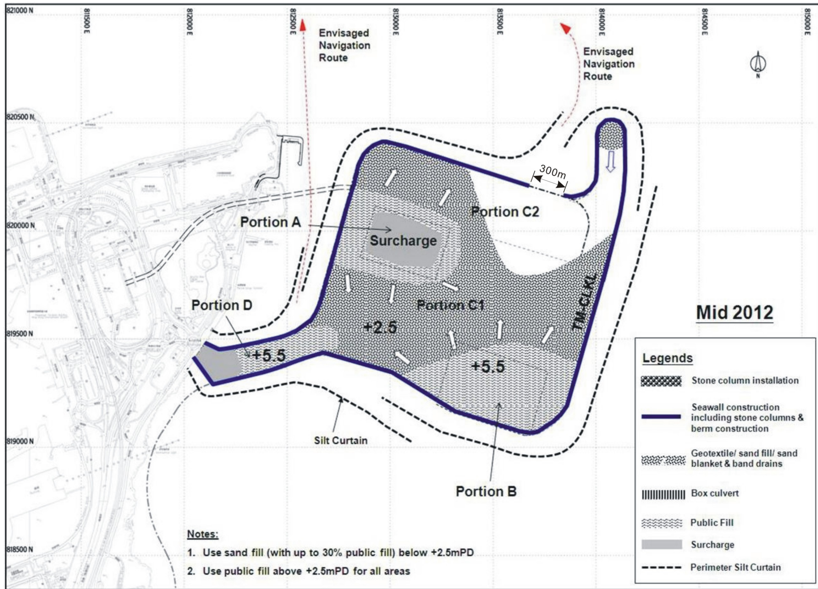
Figure 15 - Outline of Construction Sequence (Sheet 4 of 10) 圖 15 - 施工程序大綱(表10之4)
